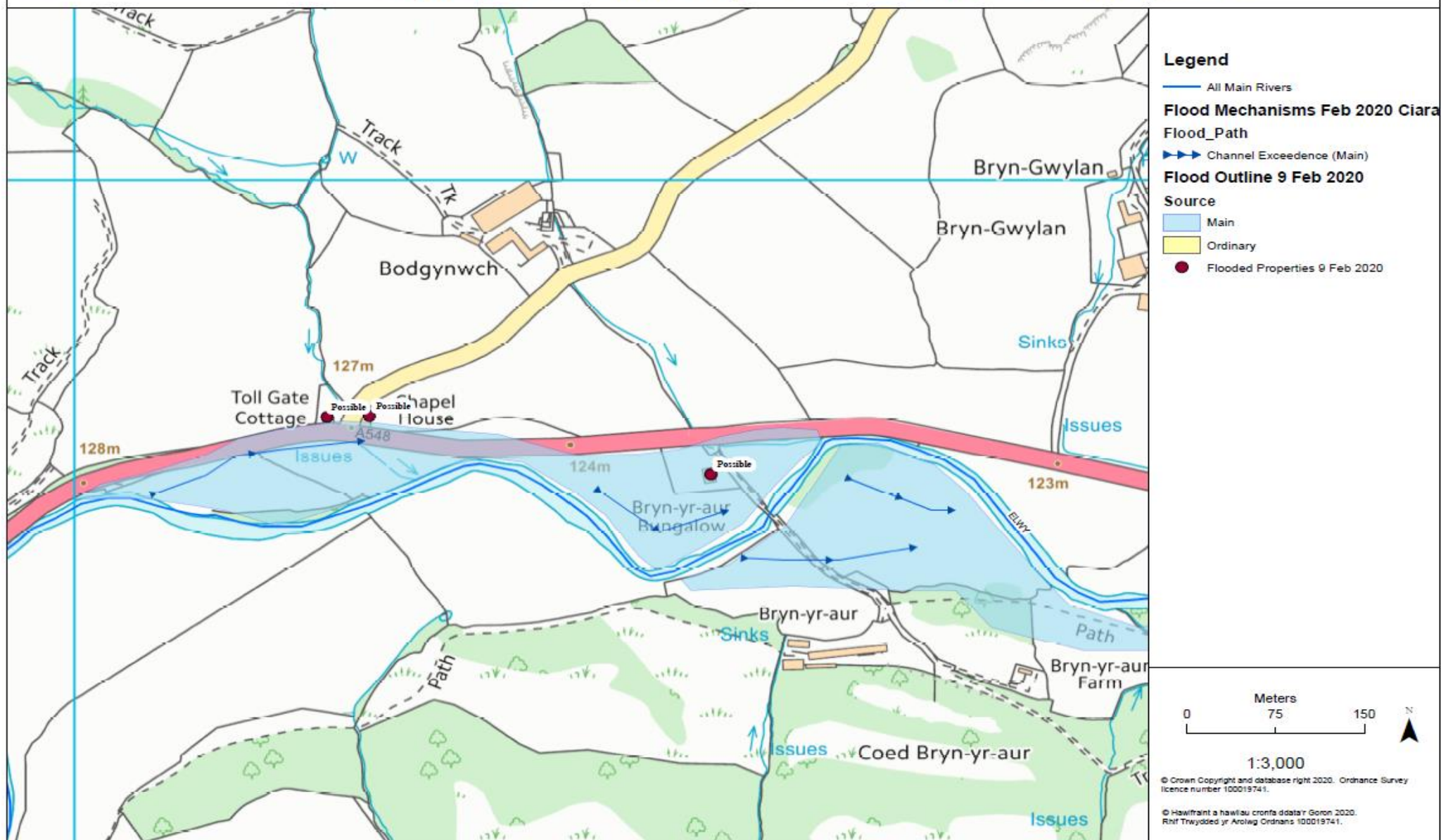
Figure 84: Bryn Yr Aur Community flood mechanisms - Feb 2020
