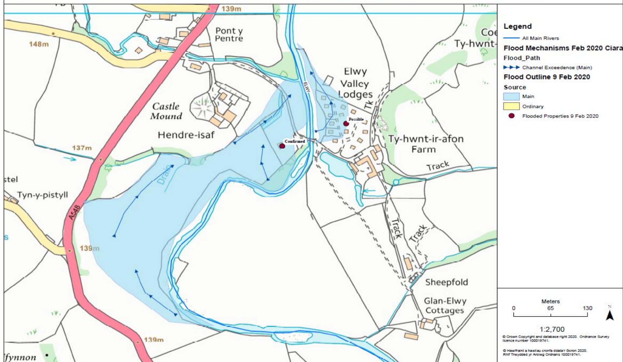
Figure 85: Hendre Isaf Community flood mechanisms - Feb 2020
