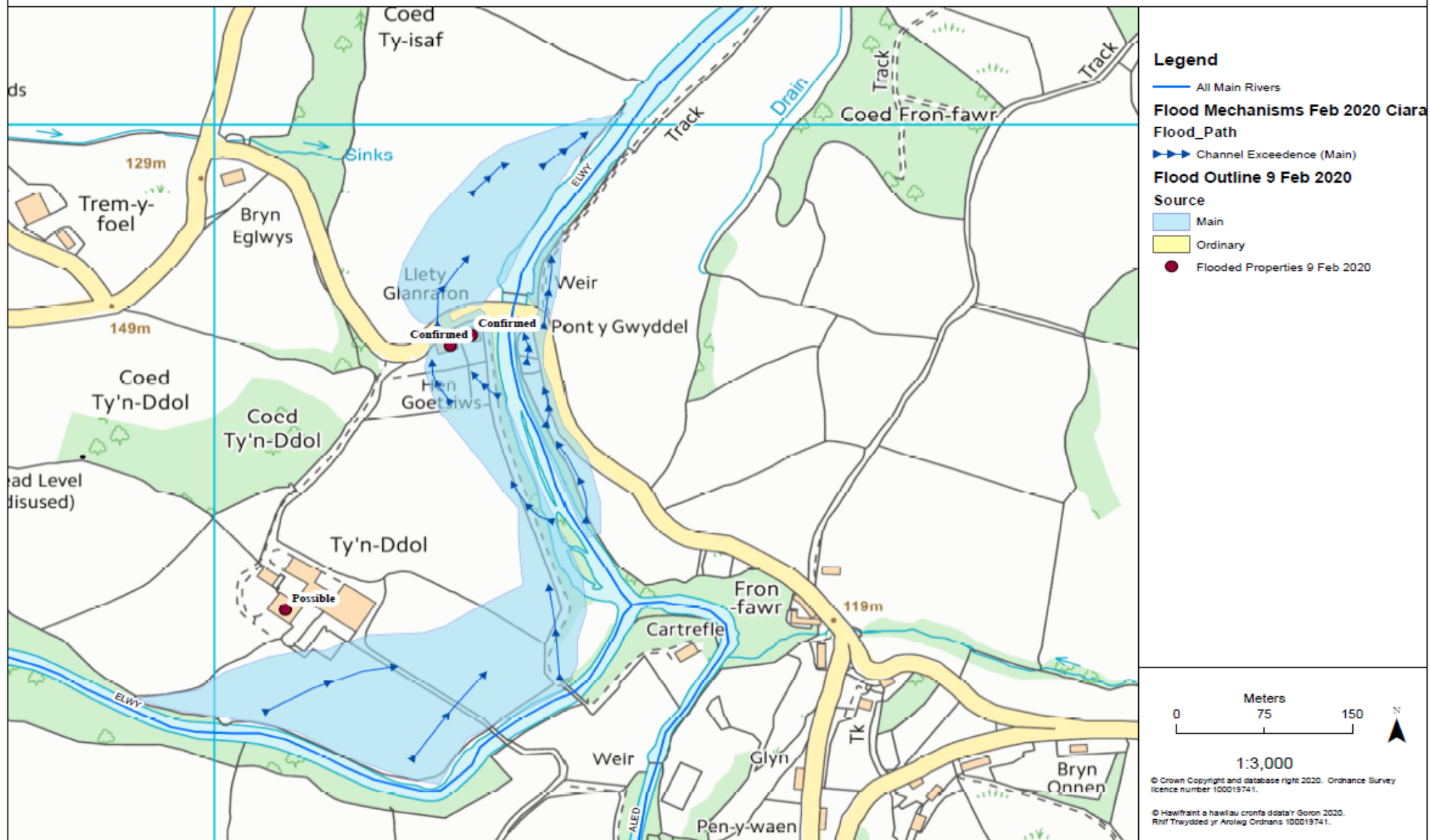
Figure 74: Pont Y Gwyddel community flood mechanisms - Feb 2020
