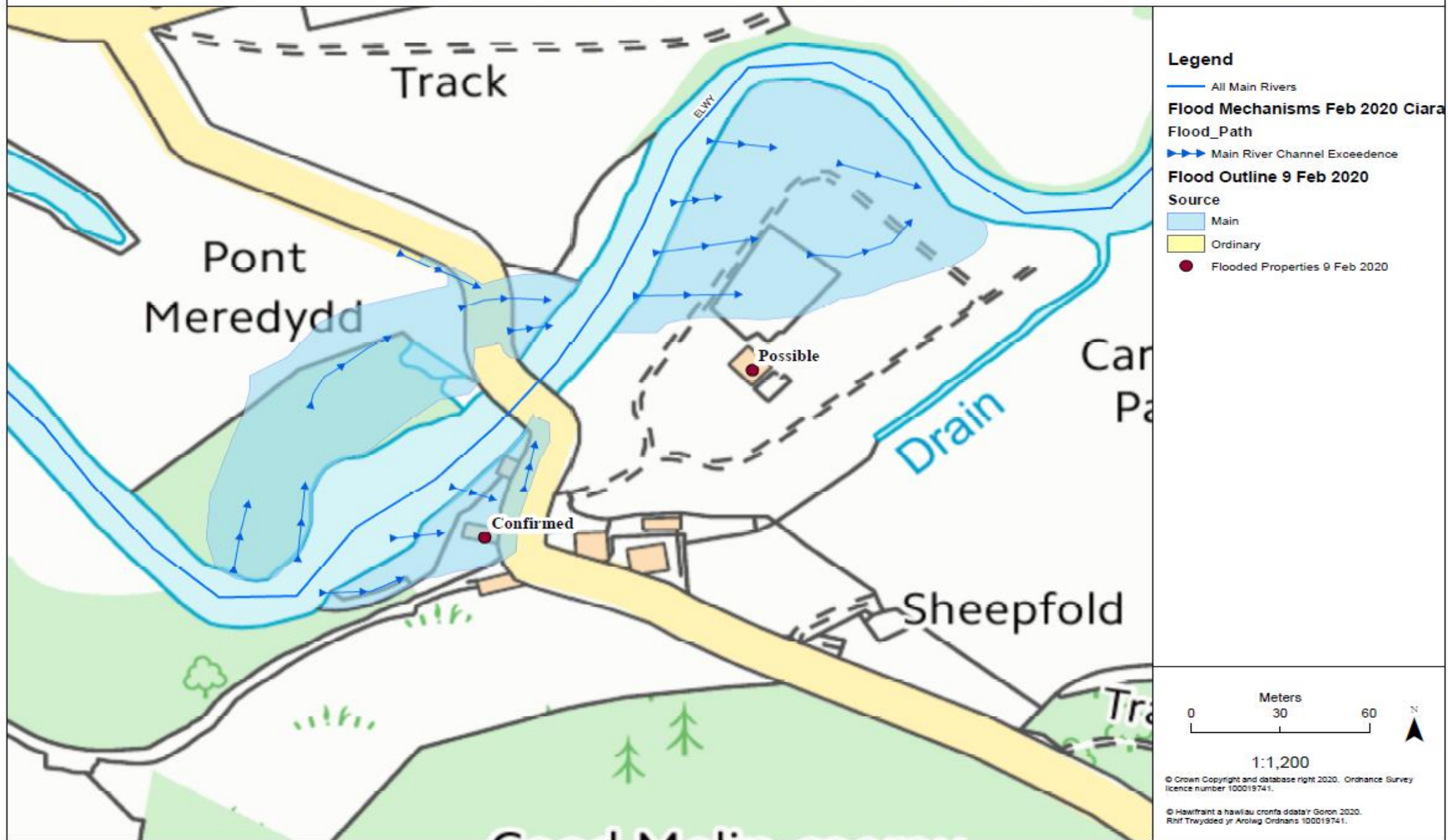
Figure 73: Pont Meredydd community flood mechanisms - Feb 2020
