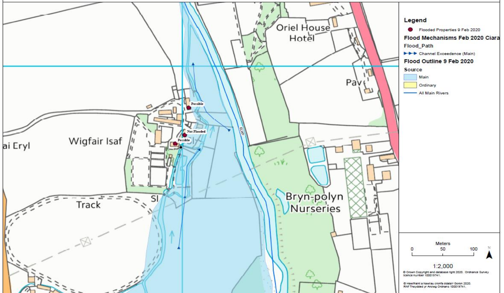
Figure 66: Wigfair Isaf community flood mechanisms - Feb 2020
