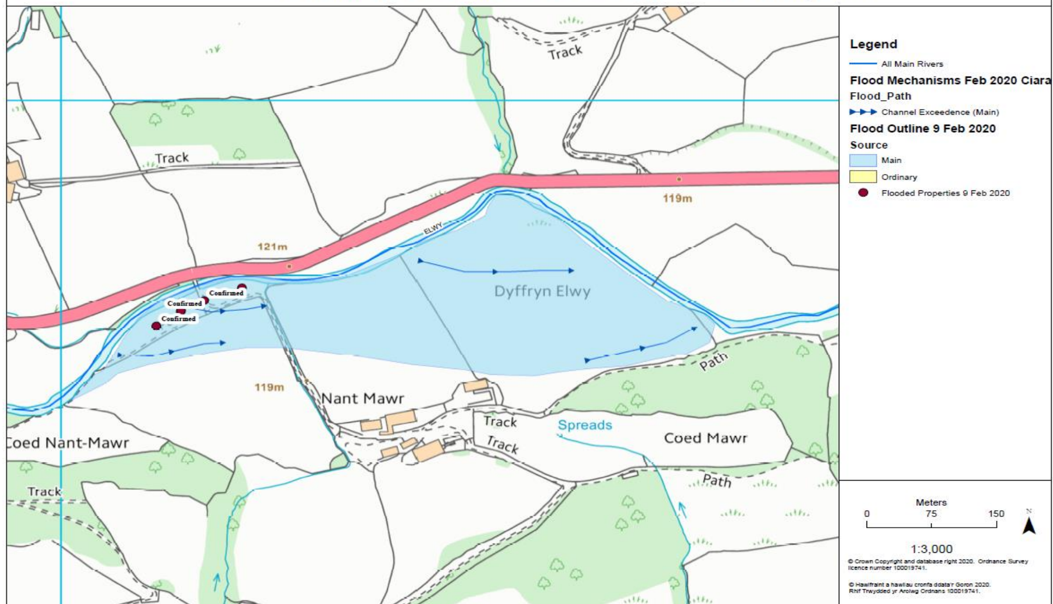
Figure 82: Nant Mawr Caravans flood mechanisms - Feb 2020
