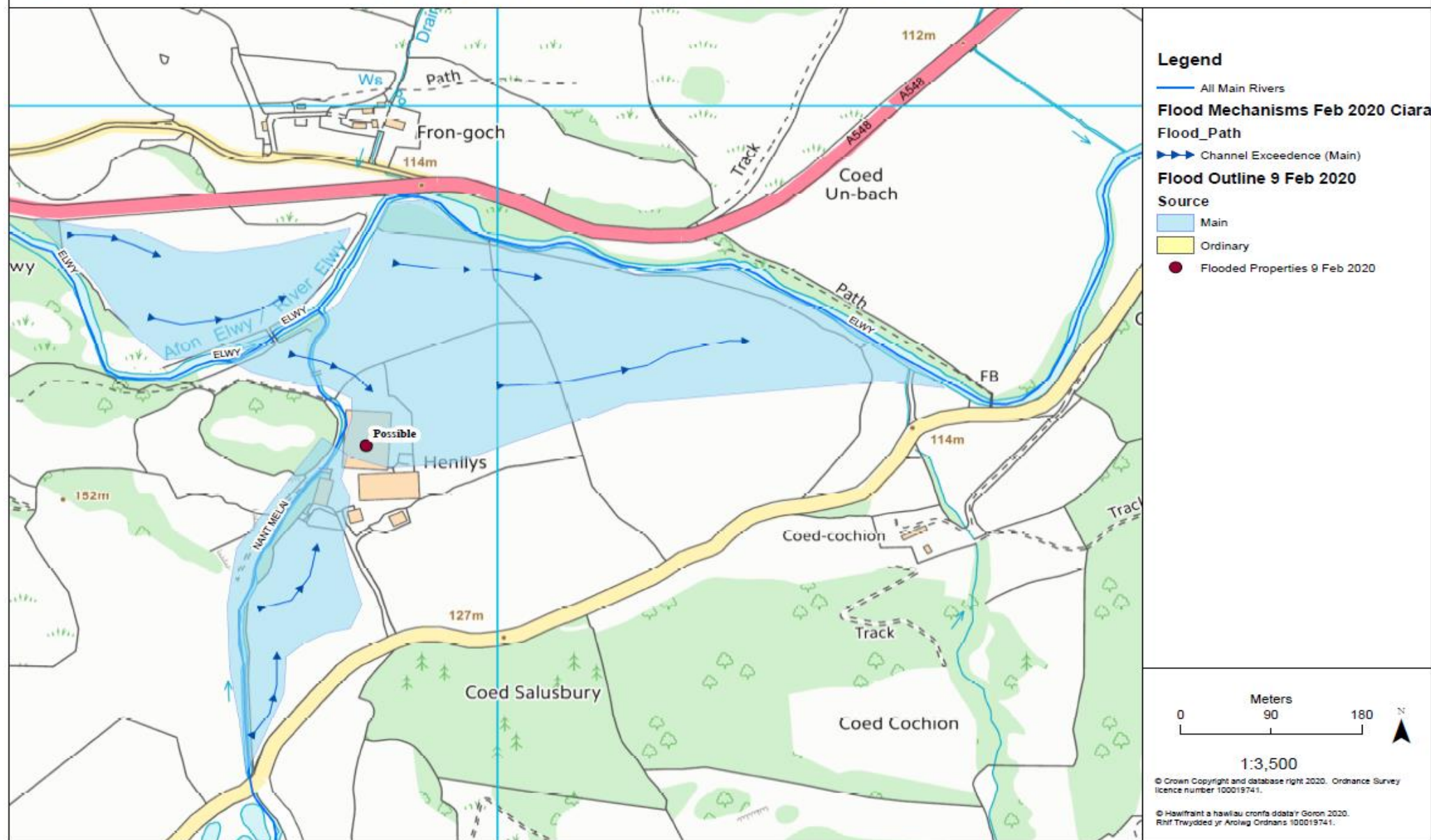
Figure 80: Henllys Farm flood mechanisms - Feb 2020
