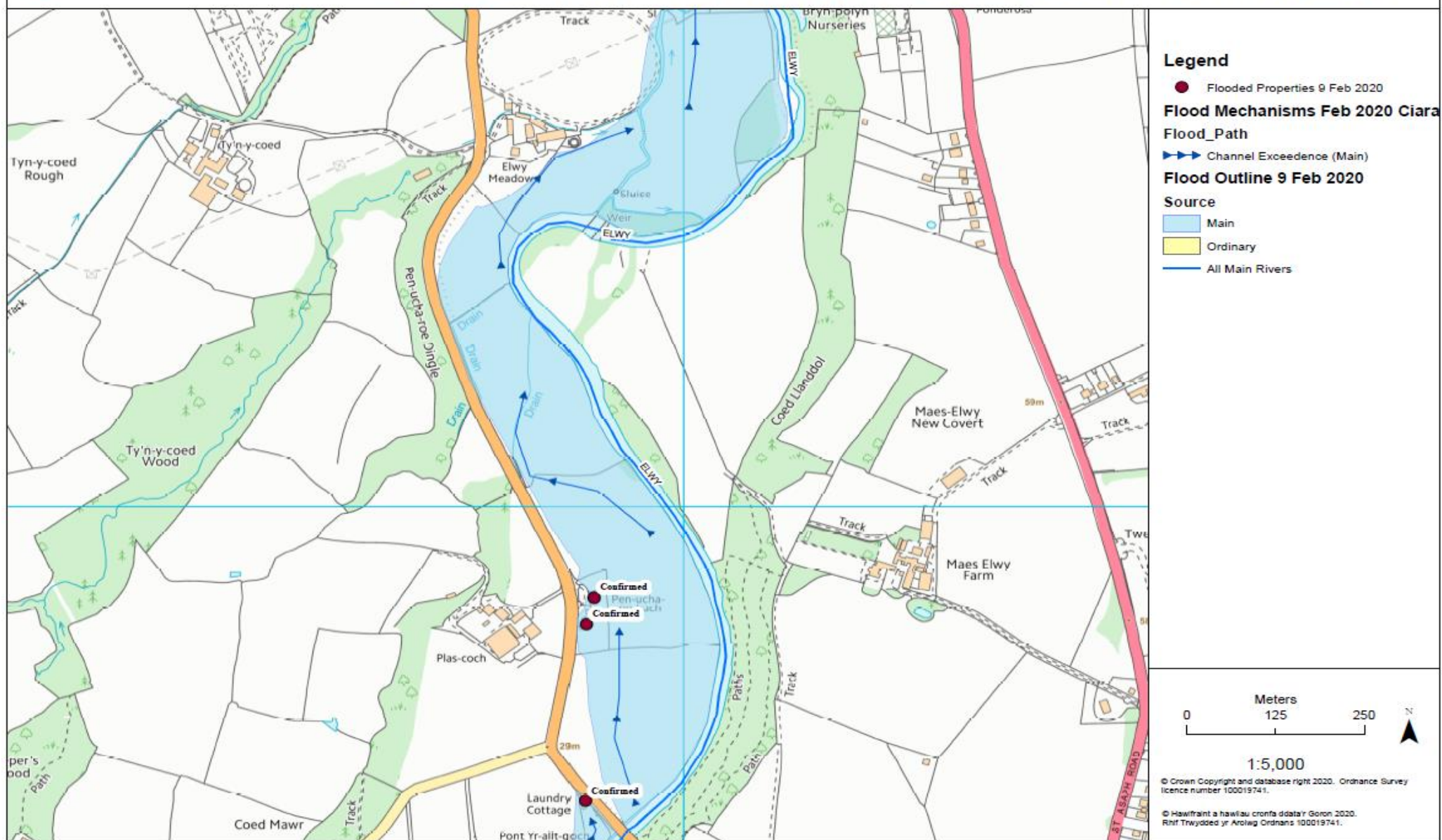
Figure 67: Lower Denbigh Road community flood mechanisms - Feb 2020
