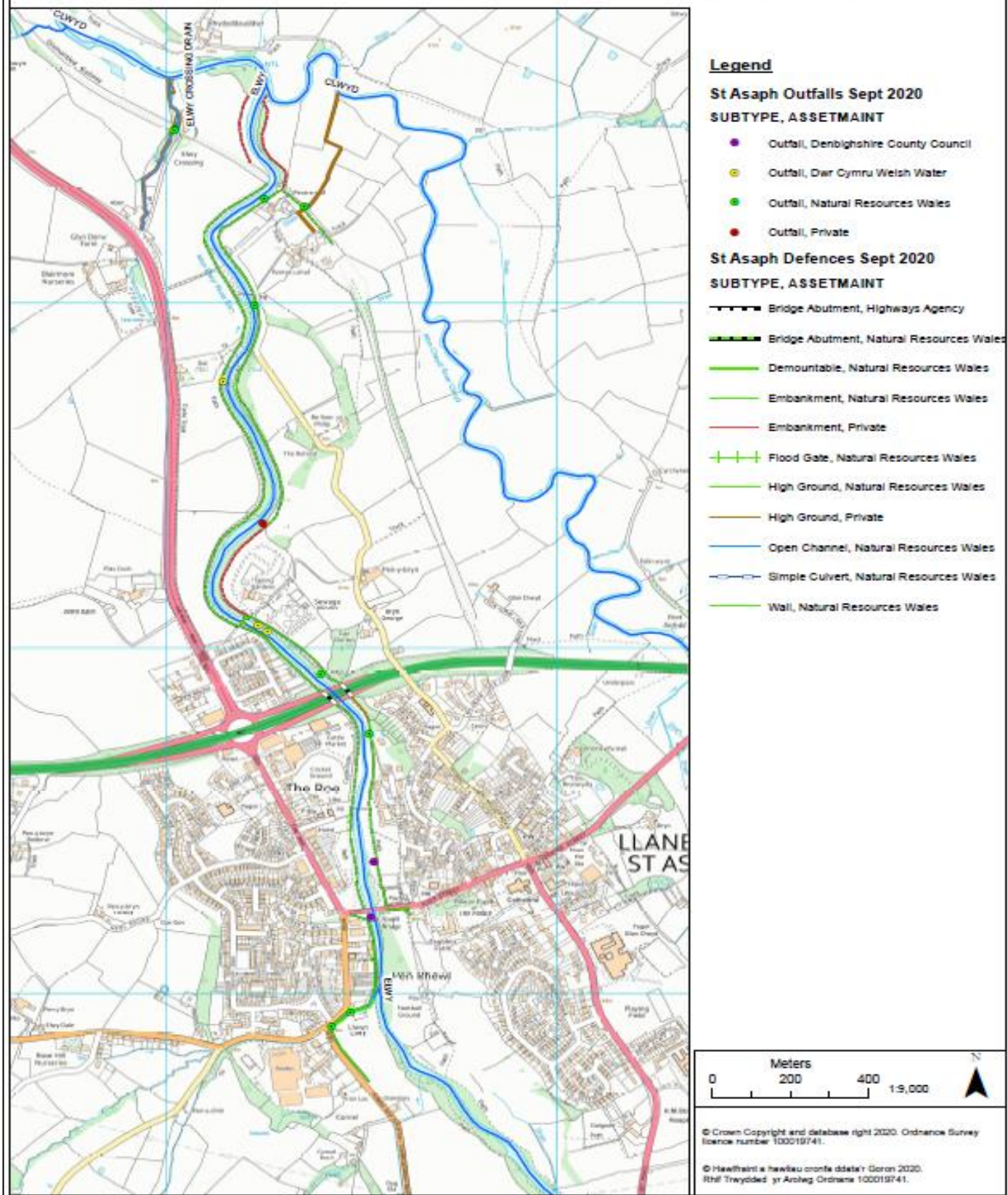
Figure 20: Overview map of St Asaph flood defences
