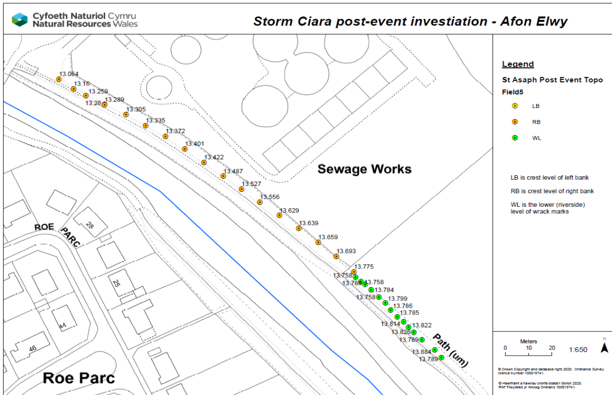
Figure 49: Post-event topographic survey (NRW, 2020)
