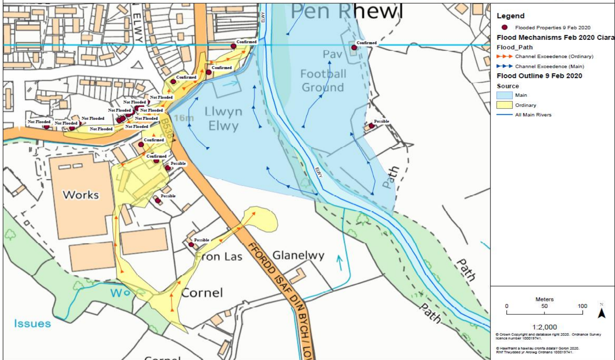
Figure 64: Glas Coed community flood mechanisms - Feb 2020
