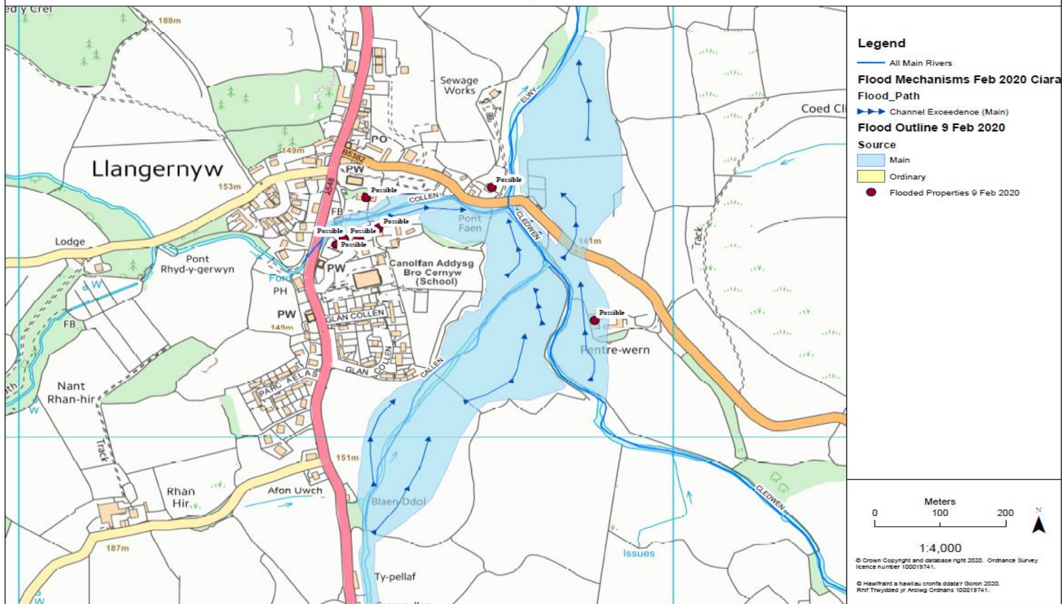
Figure 86: Llangernyw Community flood mechanisms - Feb 2020
