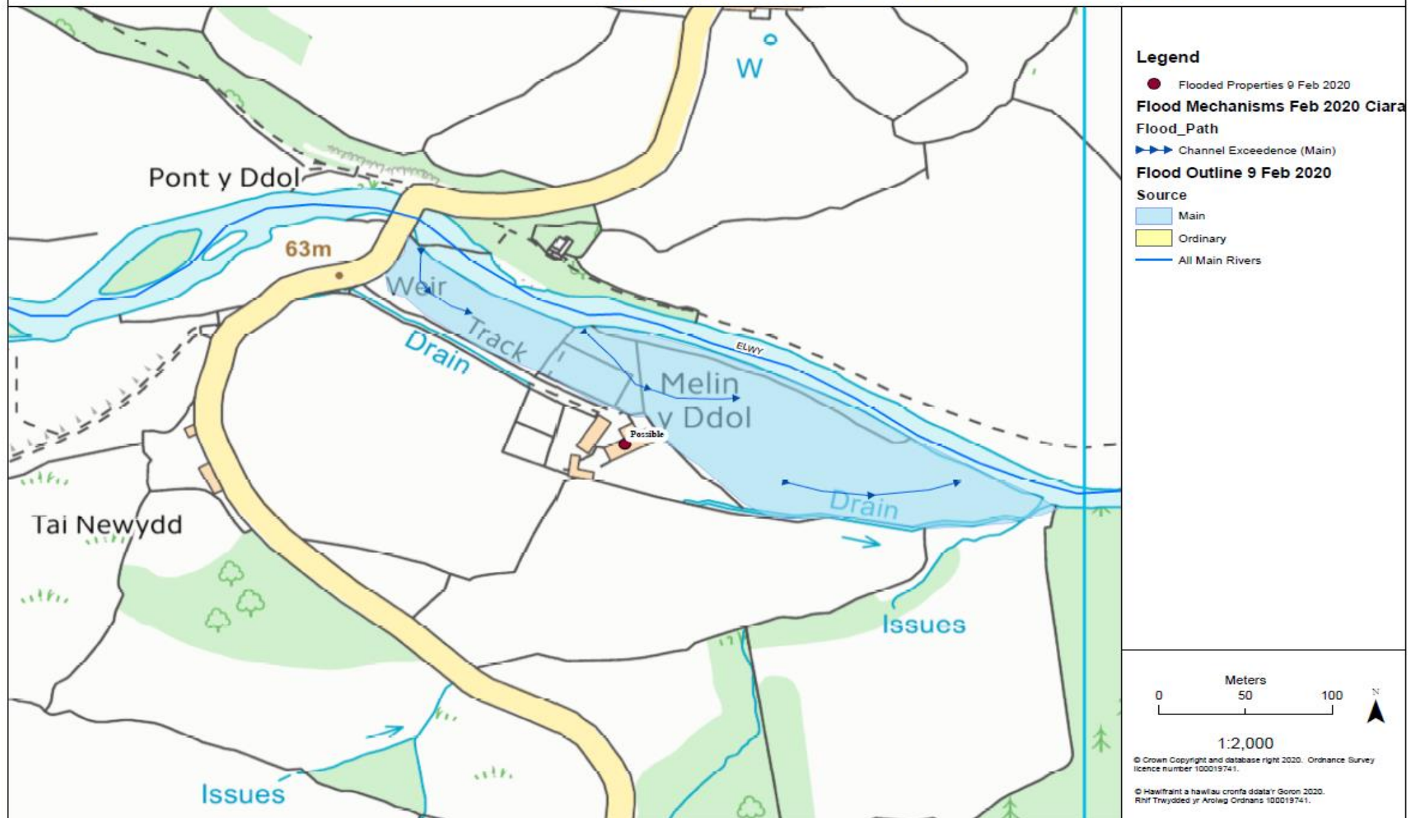
Figure 72: Pont Y Ddol community flood mechanisms - Feb 2020
