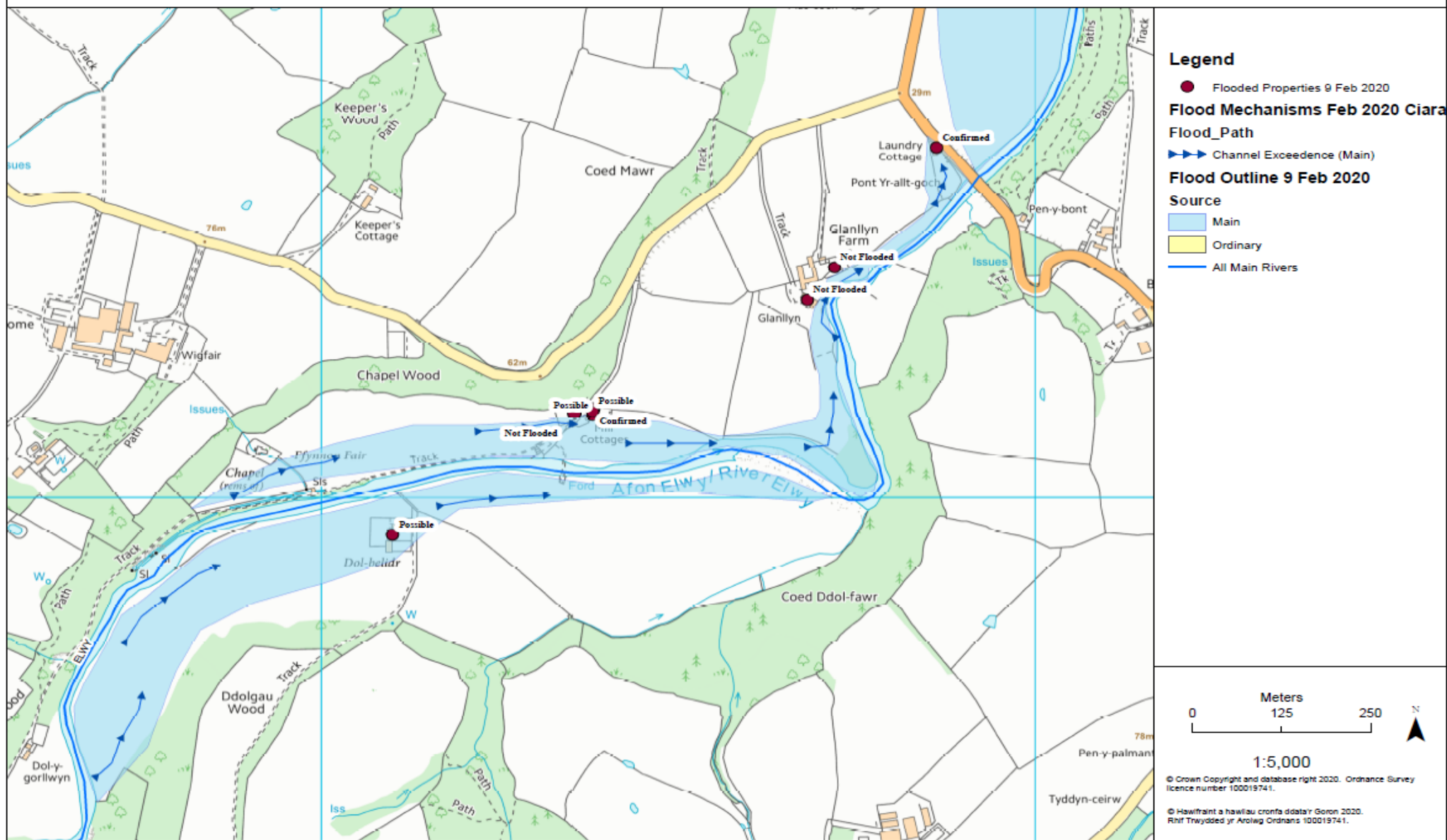
Figure 70: Chapel Wood community flood mechanisms - Feb 2020
